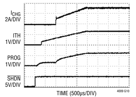
PWM Soft-Start
