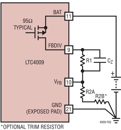
Figure 5. Programming LTC4009 Output Voltage
