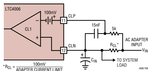
Figure 9. Adapter Current Limiting
