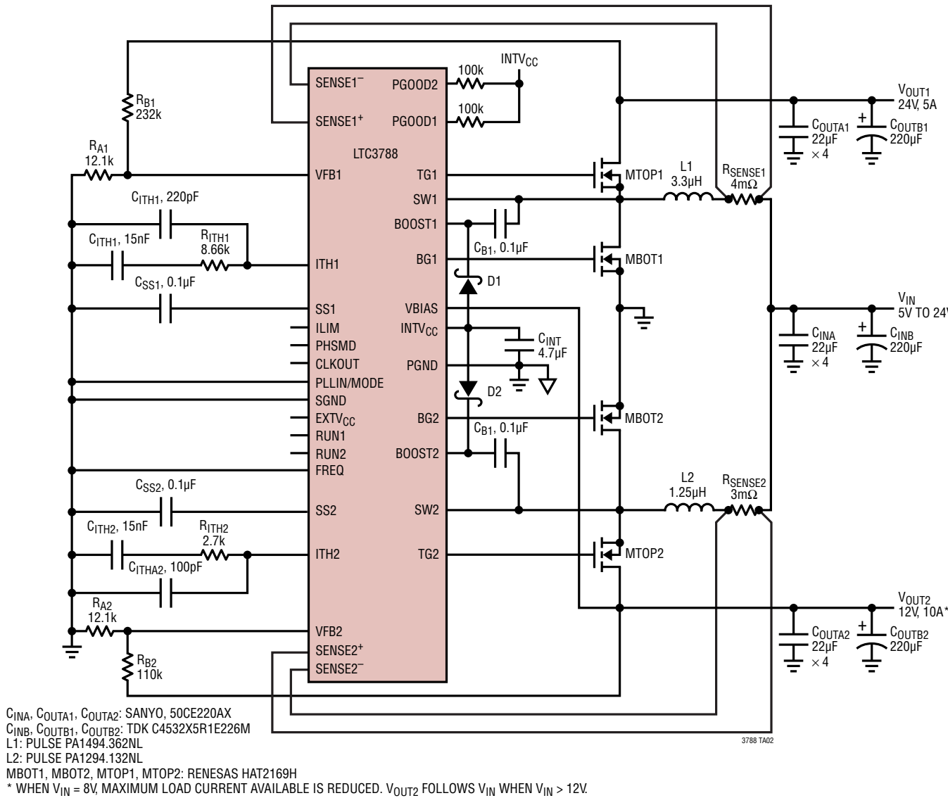
High Efficiency Dual 12V/24V Boost Converter
