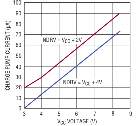
Charge Pump Output Current vs V CC Supply Current
