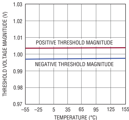
I SMAG Thresholds vs Temperature
