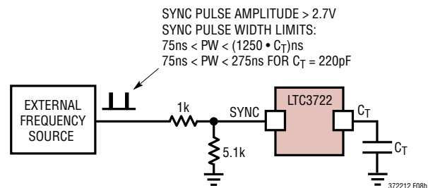
Figure 8b. SYNC Input from an External Source
