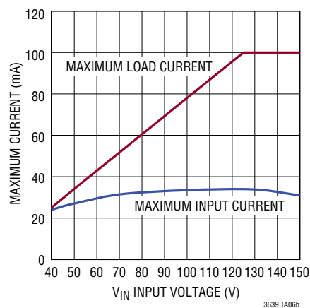
Maximum Load and Input Current vs Input Voltage
