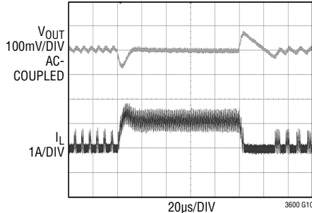
Transient Response DCM, Operation, External Compensation
