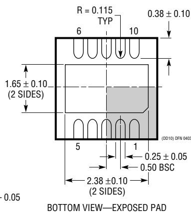
BOTTOM VIEW—EXPOSED PAD
