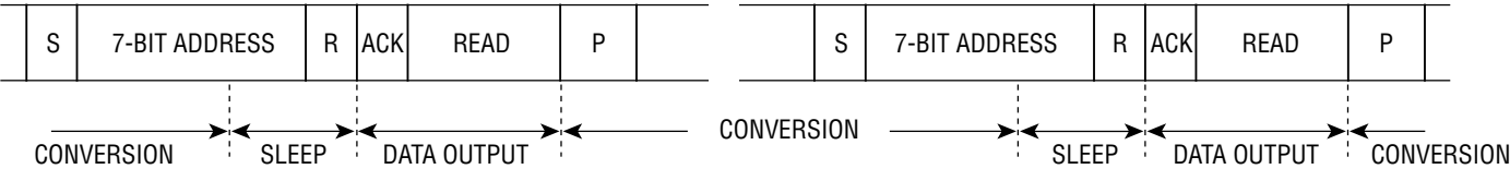
Figure 5. Consecutive Reading with the Same Input/Configuration
