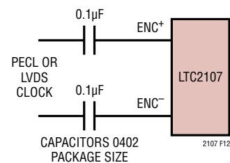
Figure 12. PECL or LVDS Encode Drive
