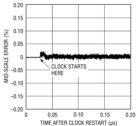
Mid-Scale Settling After Starting Encode Clock with Keep-Alive On
