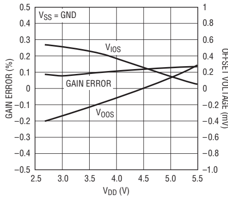
Gain and Offsets vs V_{DD} Supply
