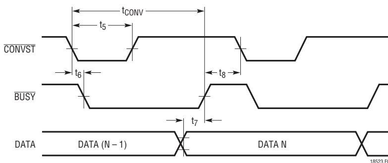
Figure 5. Mode 1a \overline{\text{CONVST}} Starts a Conversion. Data Outputs Always Enabled ( \overline{\text{CS}} = \overline{\text{RD}} = 0 )
