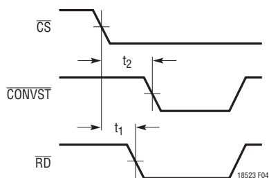
Figure 4. \overline{\text{CS}} to \overline{\text{CONVST}} and \overline{\text{RD}} Setup Timing
