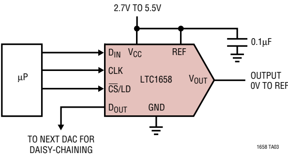
14-Bit, 3V to 5V Single Supply, Voltage Output DAC
