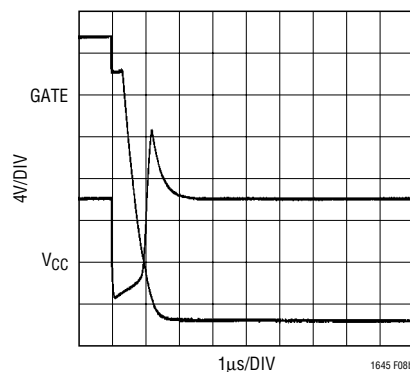
(b) V_{CC} Supply Glitch Without Any Limiting
