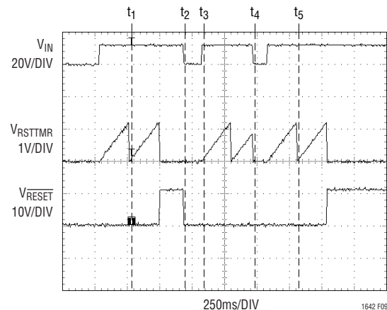
Figure 13. Supply Monitor Waveforms
