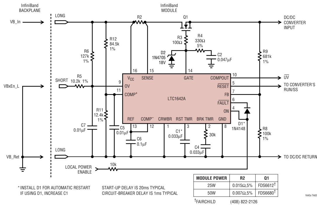
12V Hot Swap Circuit for InfiniBand Modules
