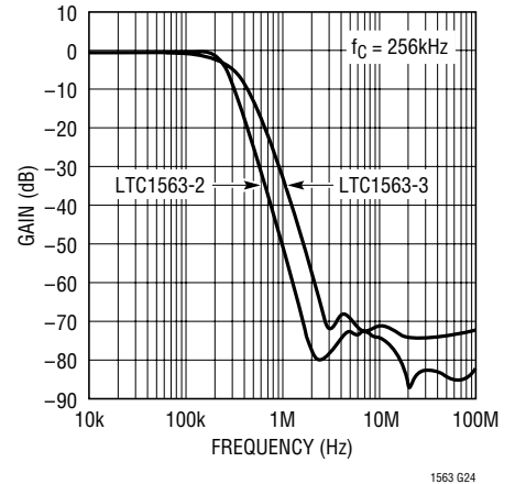
Stopband Gain vs Input Frequency
