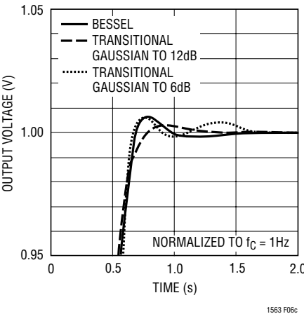
Figure 6c. Step Response—Settling
