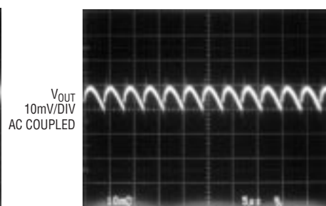
Output Ripple, C_{OUT} = 22\mu\text{F}
