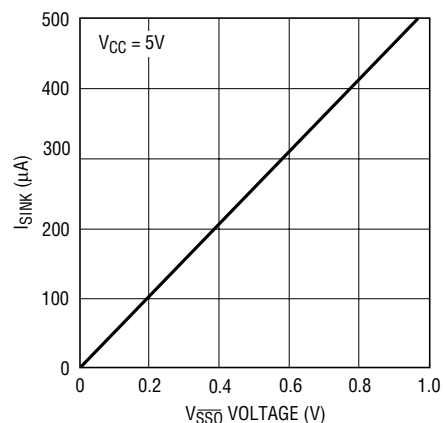
LTC1296 SS O Sink Current vs V SSO
