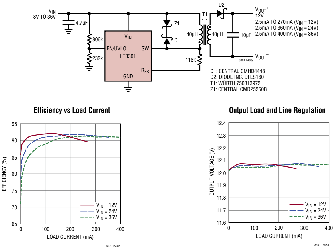
8V to 36V IN /12V OUT Micropower Isolated Flyback Converter
