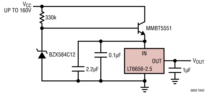
Extended Supply Range Reference
