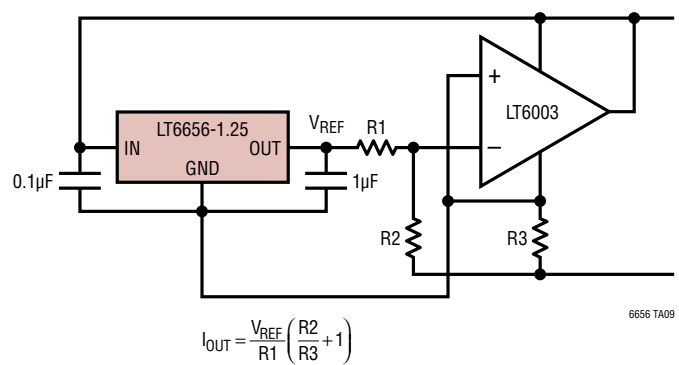
2-Terminal Current Source
