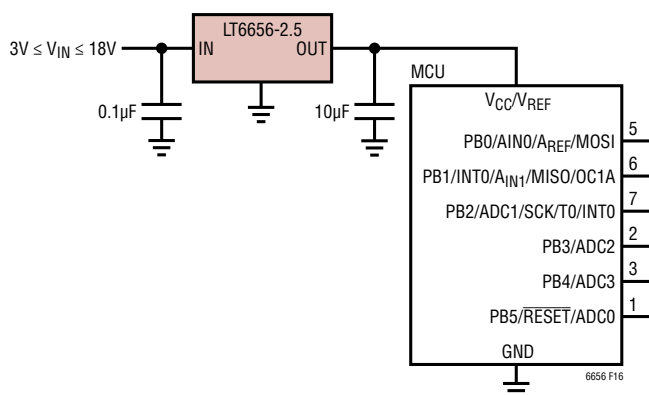
Figure 16. Microcontroller Reference and Regulator
