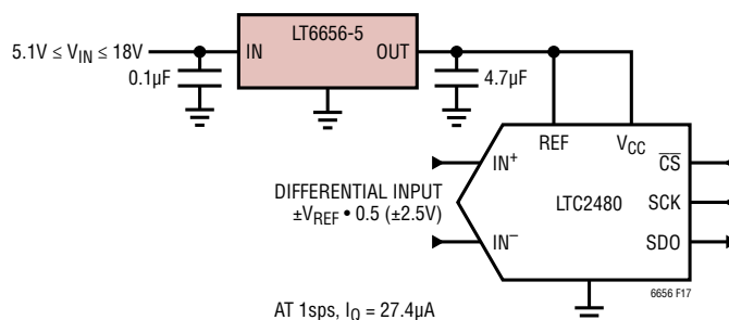
Figure 17. Low Power ADC Reference
