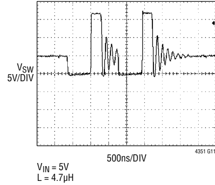
Typical SW Pin Waveform
