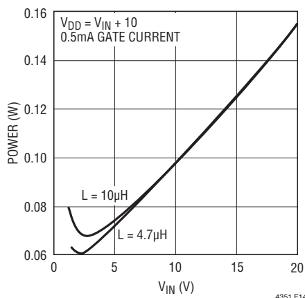
Figure 14. Total Power (Typical)
