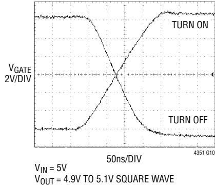
GATE Pin Turn On and Off Waveform with 10nF Capacitor Load
