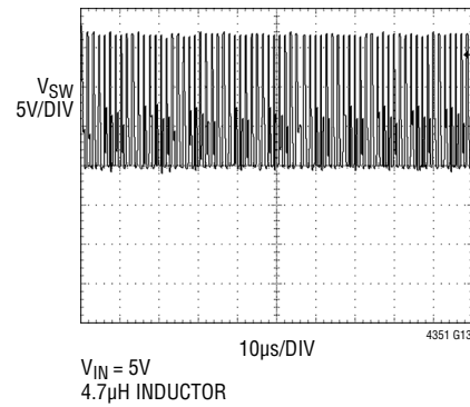
SW Pin Waveform at Maximum Boost Regulator Output
