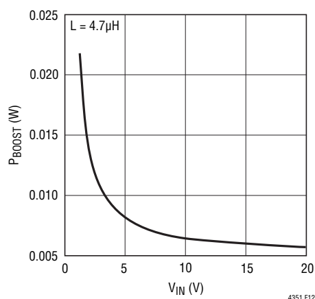
Figure 12. P_{BOOST}(TYP)
