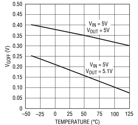
Gate Off-Voltage vs Temperature
