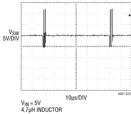
Typical SW Pin Waveform
