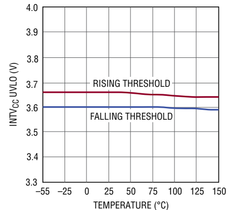
INTV_{CC} Undervoltage Lockout vs Temperature
