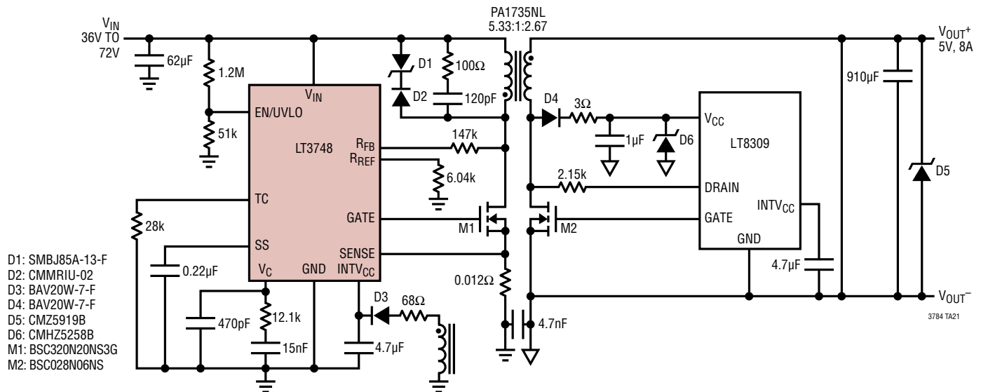
Figure 21. 5V, 8A Isolated Supply with Synchronous Secondary-Side Rectification Using LT309
