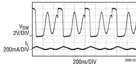
Fixed Frequency No Load Waveform
