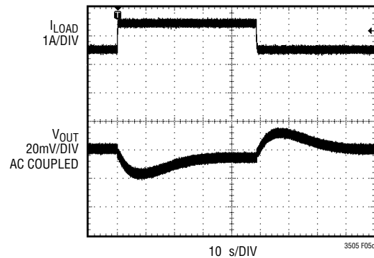
Figure 5. Transient Load Response of the LT3505 with Different Output Capacitors as the Load Current is Stepped from 500mA to 1.2A. V IN = 12V, V OUT = 3.3V, L = 2μH, R T = 20.0k
