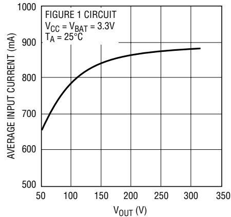
Input Current, LT3420
