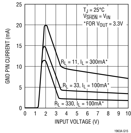
LT1963A-3.3 GND Pin Current
