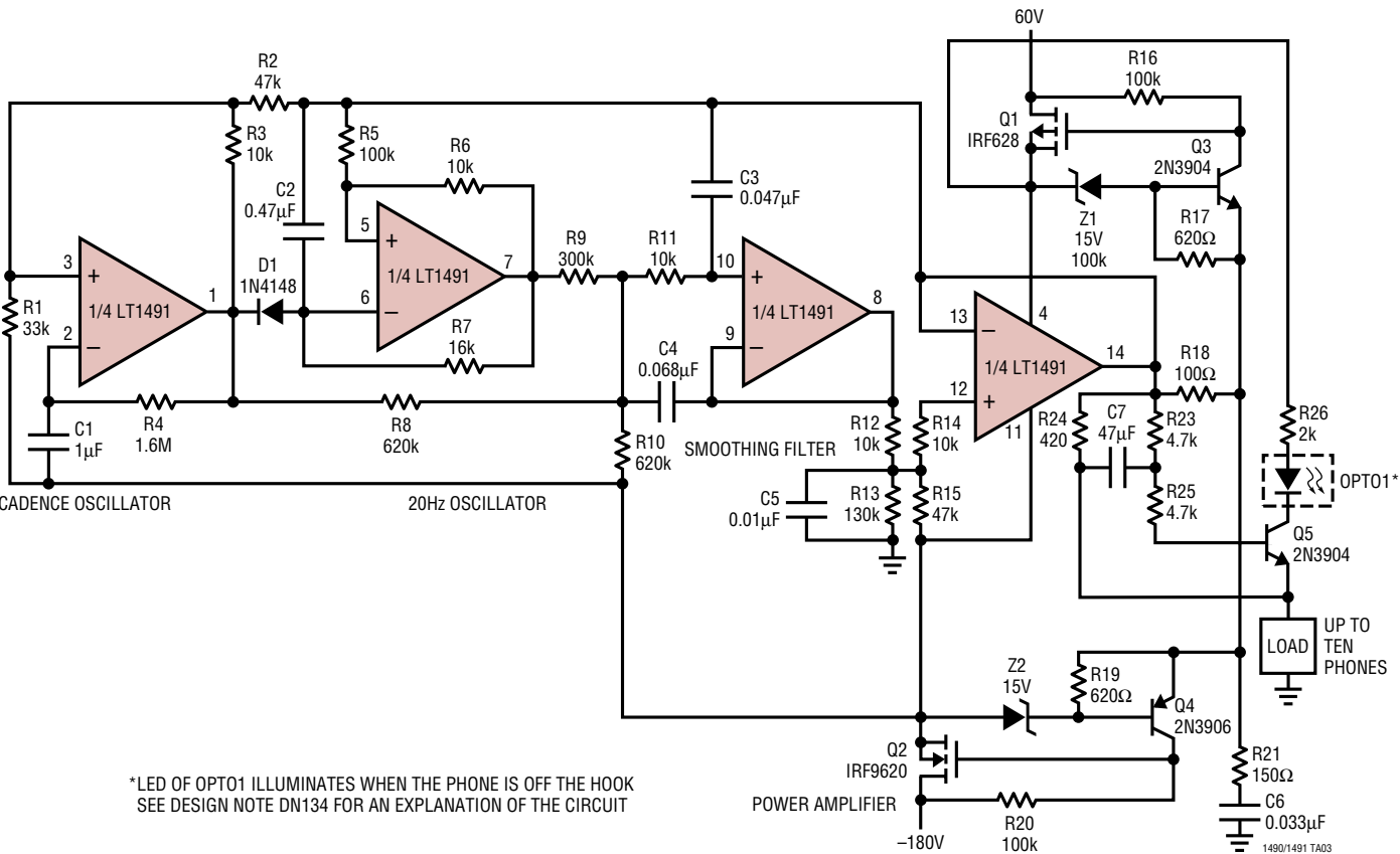
Ring-Tone Generator
