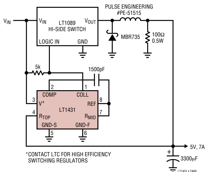
12V to 5V Buck Converter with Foldback Current Limit*
