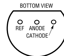
Z PACKAGE 3-LEAD TO-92 PLASTIC T_J \text{ MAX} = 100^\circ\text{C} , \theta_{JA} = 150^\circ\text{C/W}
