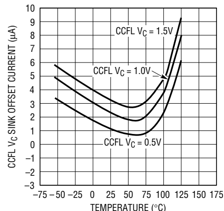
CCFL V_C Offset Sink Current vs Temperature
