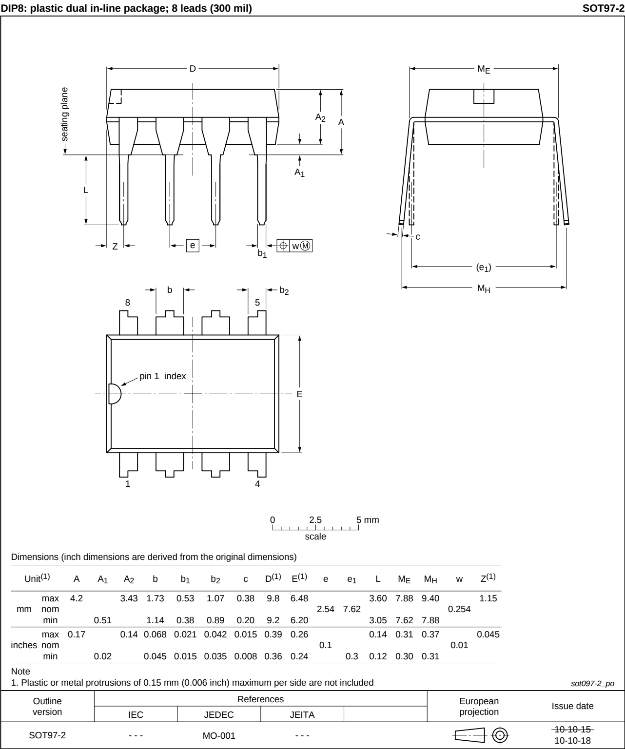
Fig 38. Package outline SOT97-2 (DIP8)
