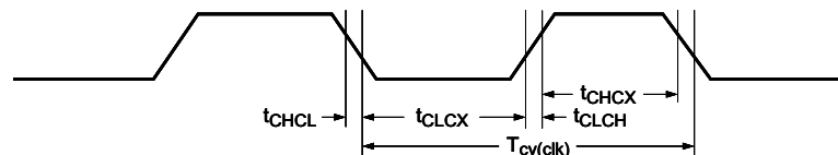
Fig 29. External clock timing (with an amplitude of at least V_{i(RMS)} = 200\text{ mV} )
