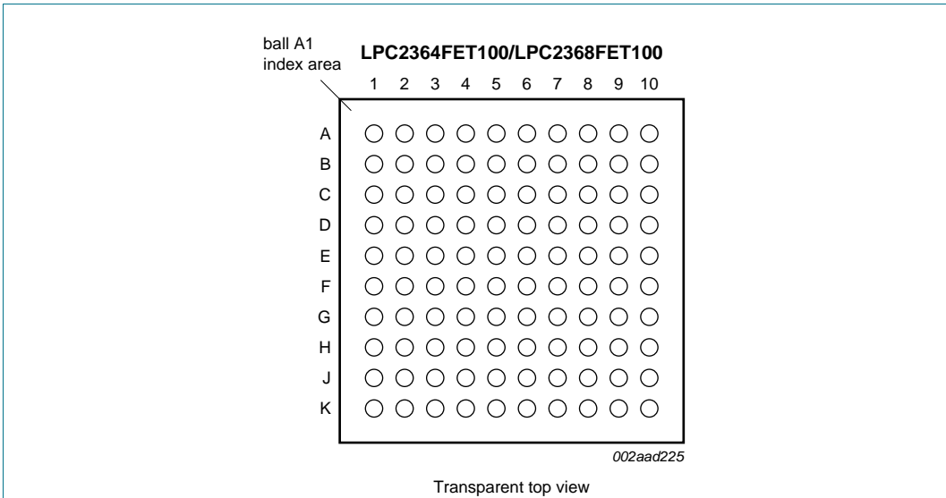
Fig 3. LPC2364/68 pinning TFBGA100 package
