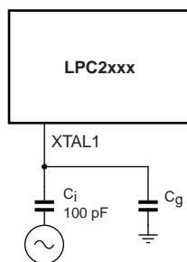
Fig 20. Slave mode operation of the on-chip oscillator
