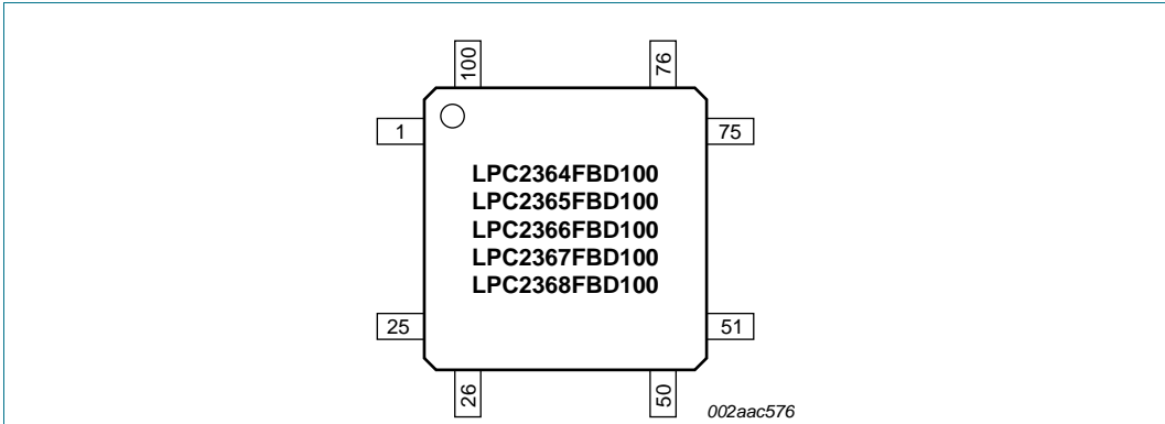
Fig 2. LPC2364/65/66/67/68 pinning
