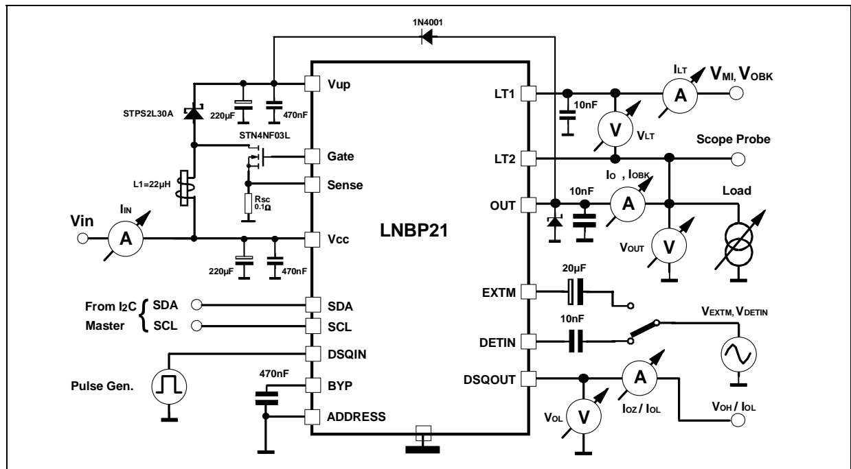
Figure 7: Test Circuit
