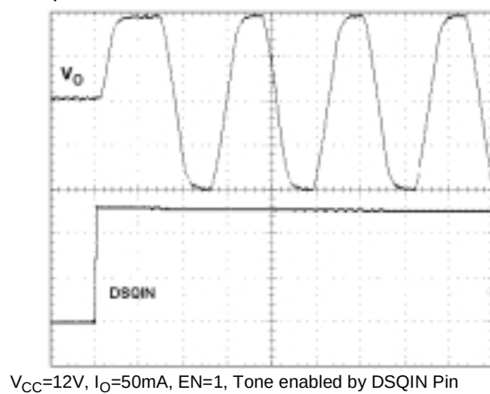
Figure 27 : DSQIN Tone Enable Transient Response
