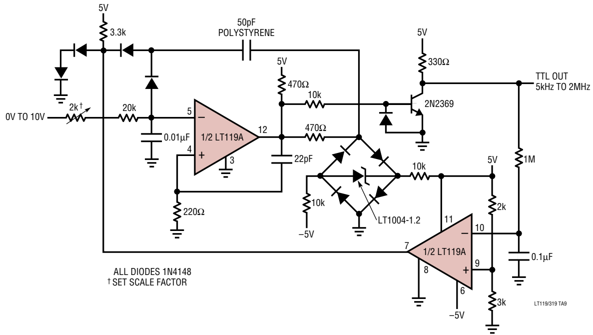
5kHz to 2MHz V \rightarrow F Converter
