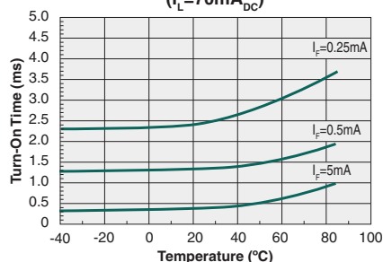
Typical Turn-On time vs. Temperature ( I_L=70\text{mA}_{\text{DC}} )
