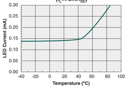
Typical I_F for Switch Operation vs. Temperature ( I_L=70\text{mA}_{\text{DC}} )
