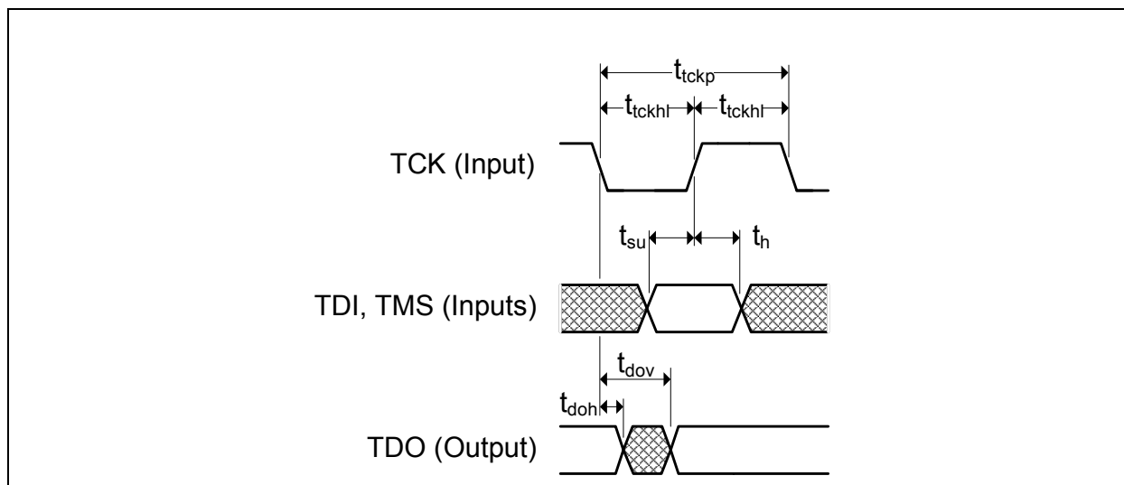
FIGURE 4-3: JTAG TIMING
