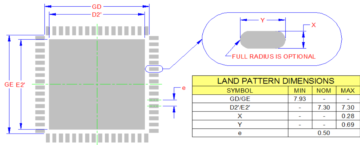
FIGURE 5-2: LAN9514/LAN9514I RECOMMENDED PCB LAND PATTERN
