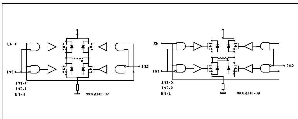
Figure 8c: Enable Chopping
