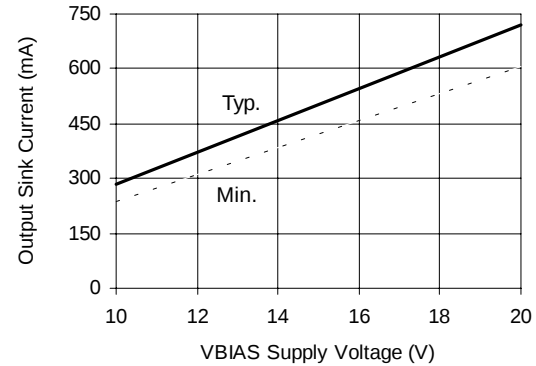
Figure 30B Output Sink Current vs Voltage
