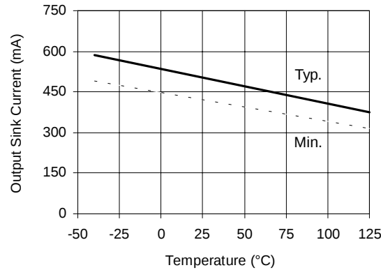
Figure 30A Output Sink Current vs Temperature
