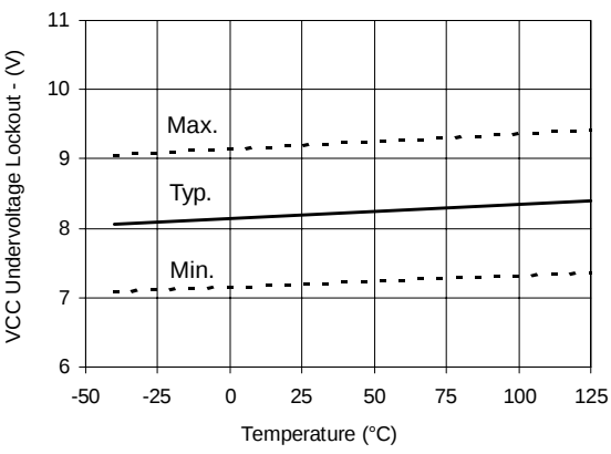
Figure 28 Vcc Undervoltage (-) vs Temperature
