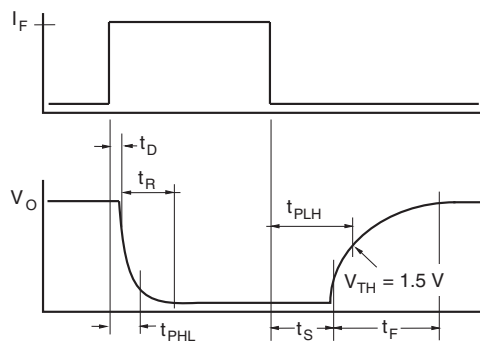
Fig. 6 - Saturated Switching Timing
