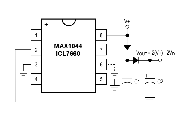
Figure 9. Voltage Doubler
