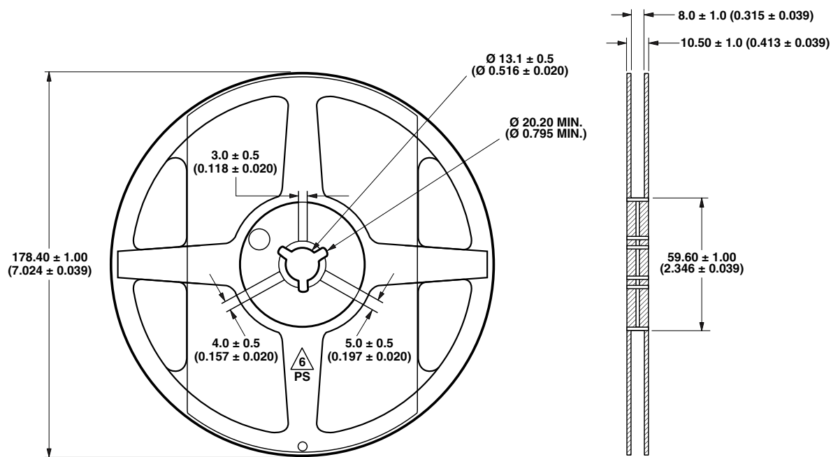
Figure 20. Reel dimensions.
