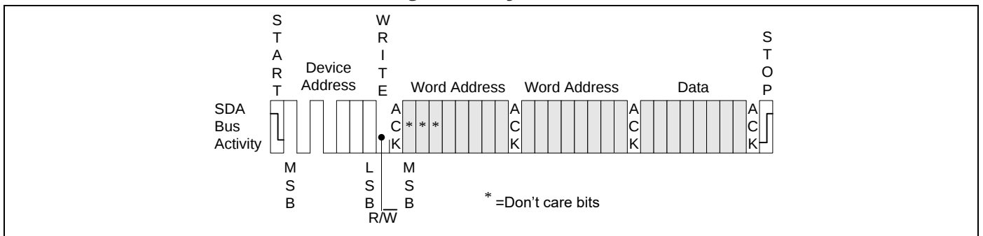
Figure 5-6. Byte Write
