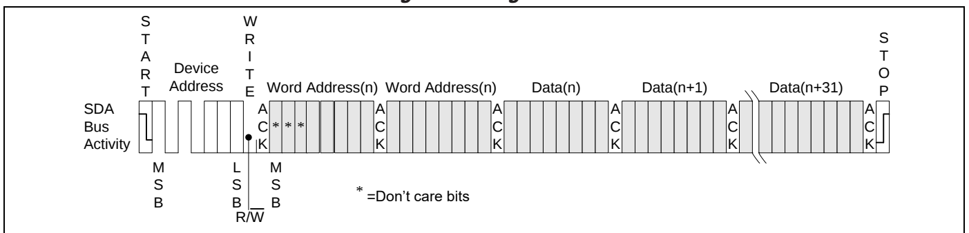
Figure 5-7. Page Write
