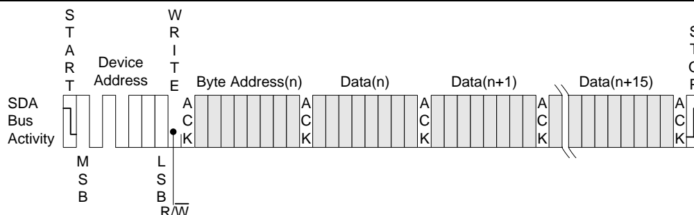
Figure 5-7. Page Write
