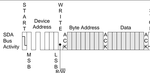
Figure 5-6. Byte Write
