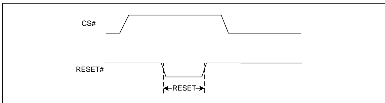
Figure2. RESET Condition
