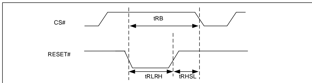
Figure49. RESET Timing
