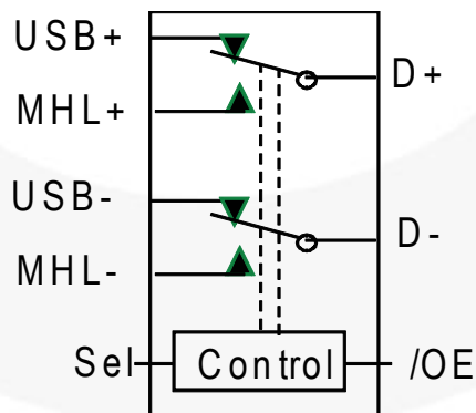
Figure 1. Analog Symbol
