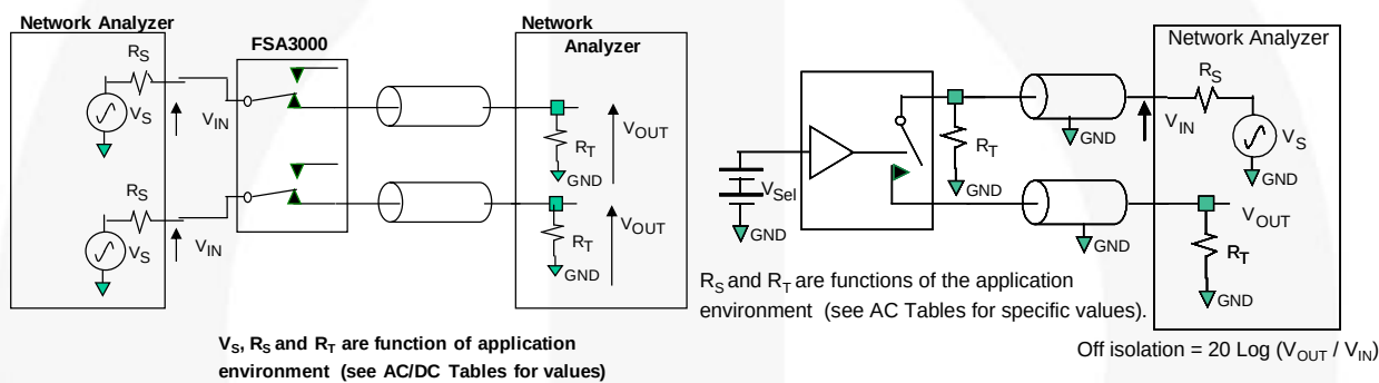
Figure 10. Insertion Loss
