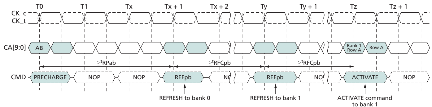
Figure 47: Per-Bank REFRESH Operation
