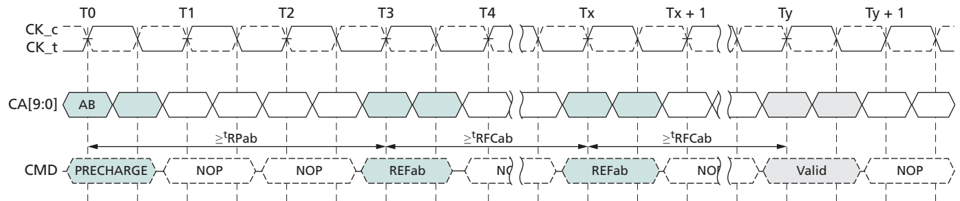
Figure 46: All-Bank REFRESH Operation
