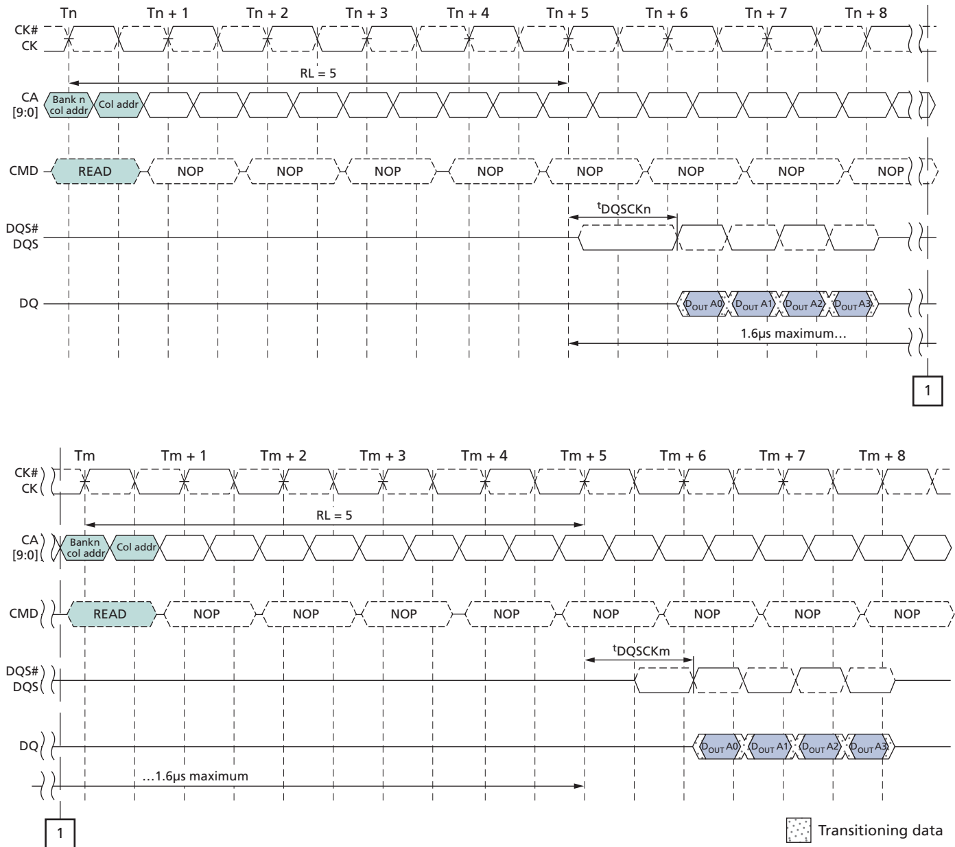
Figure 22: t_{DQSCDM} Timing
