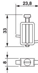
Dimensional drawing
