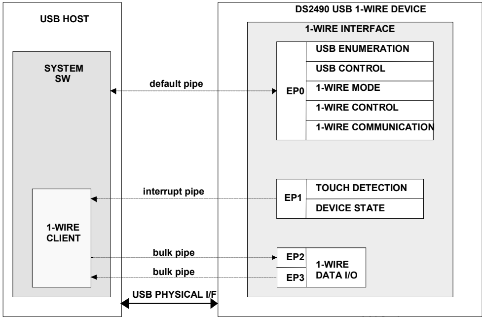
USB CONFIGURATION Figure 9
