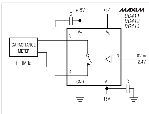
Figure 8. Channel On-Capacitance
