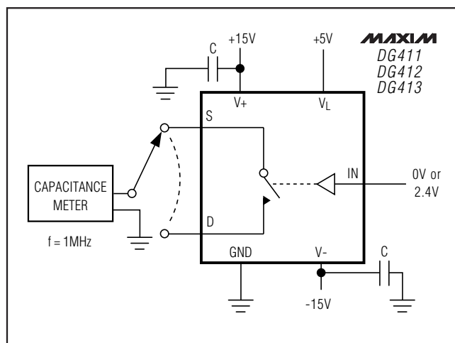
Figure 7. Channel Off-Capacitance
